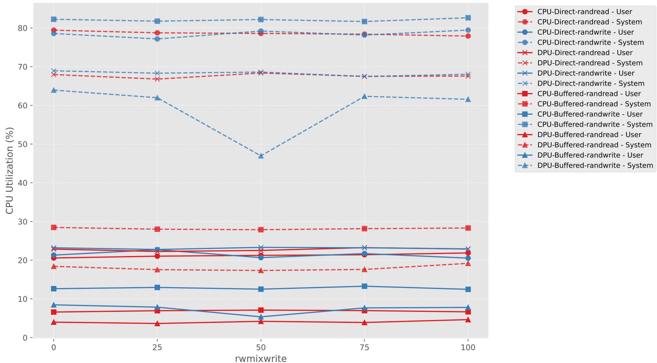
CPU Utilization vs rwmixwrite (CPU vs DPU, Direct vs Buffered)
